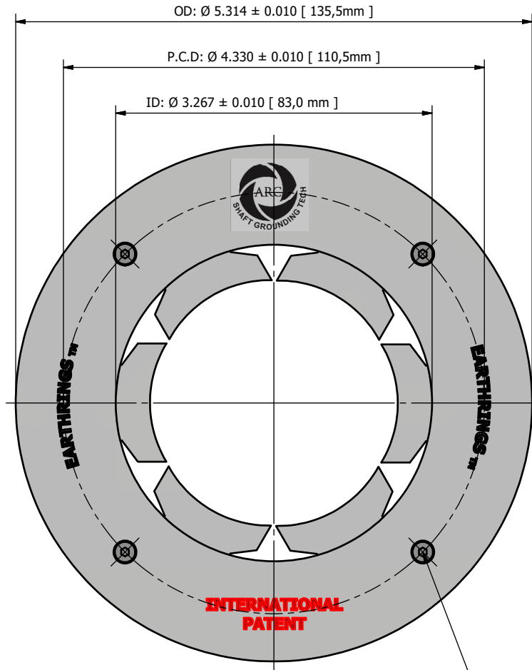
Front Plate ( 1 : 1 )
